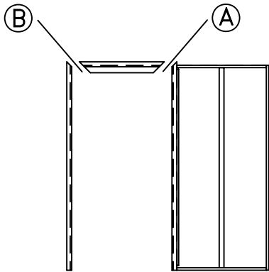
□ SINGLE POCKET — HEAD AND JAMB SHIPPED LOOSE. POCKET WELDED TO SPLIT JAMBS.
