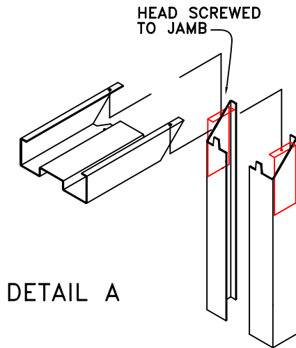
□ SINGLE POCKET — HEAD AND JAMB SHIPPED LOOSE. POCKET WELDED TO SPLIT JAMBS.
