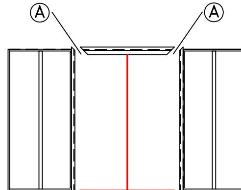
□ DOUBLE POCKET — HEAD SHIPPED LOOSE. POCKETS WELDED TO JAMBS.
