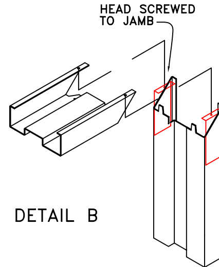
□ DOUBLE POCKET — HEAD SHIPPED LOOSE. POCKETS WELDED TO JAMBS.
