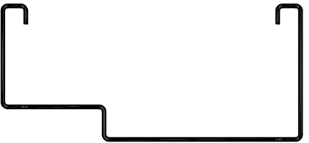
Single Rabbet w/ Drywall Returns
